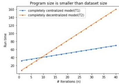
Figure 2: Program size is smaller than dataset size
